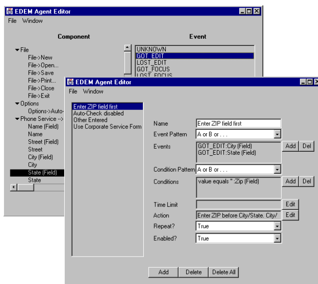
Figure 3. A simple agent editor.
